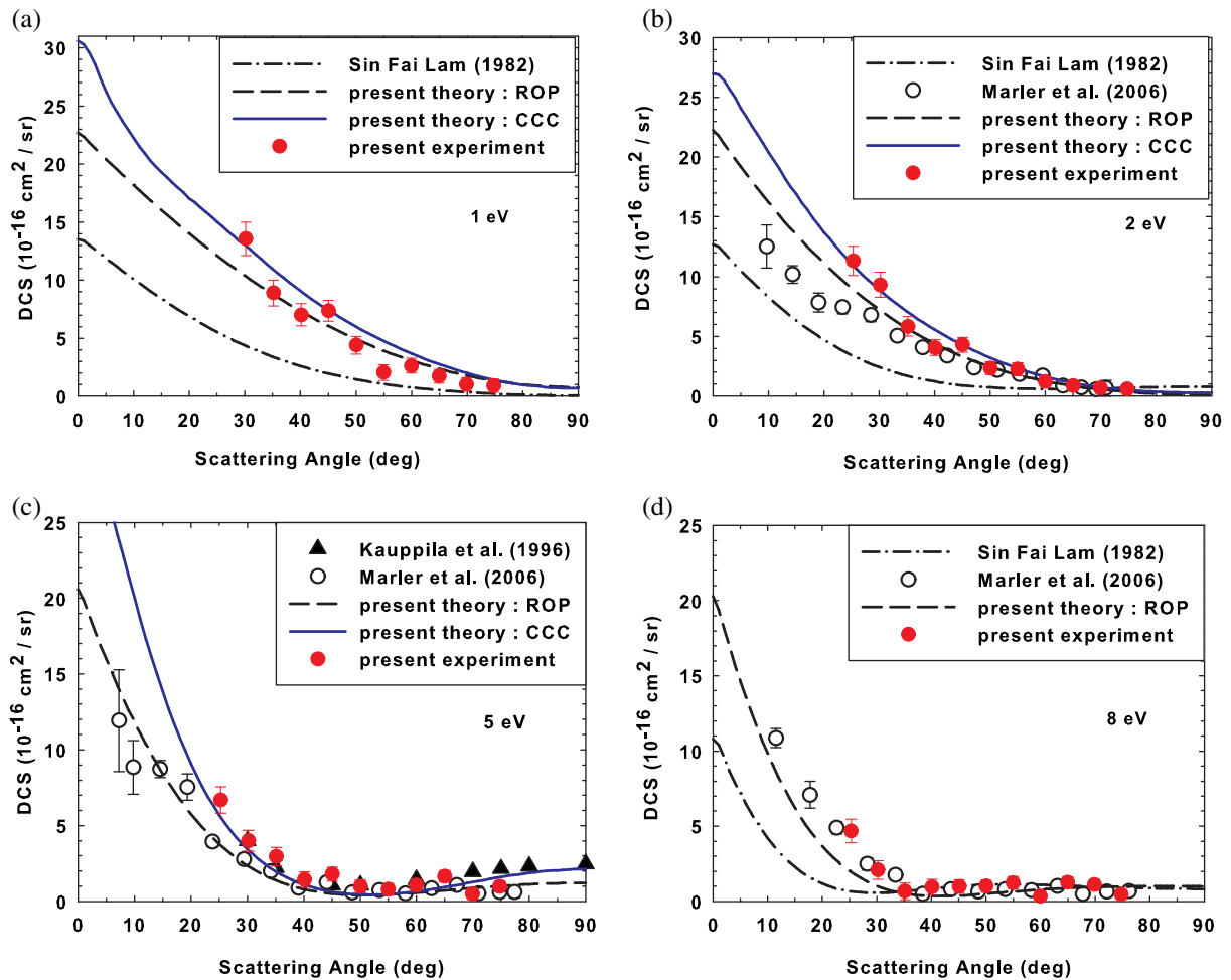
Figure 3. Absolute elastic DCS ( 10^{-16} \text{ cm}^2 \text{ sr}^{-1} ) for positron scattering from Xe compared with experimental and theoretical values from the literature at energies from 1 to 8 eV.
