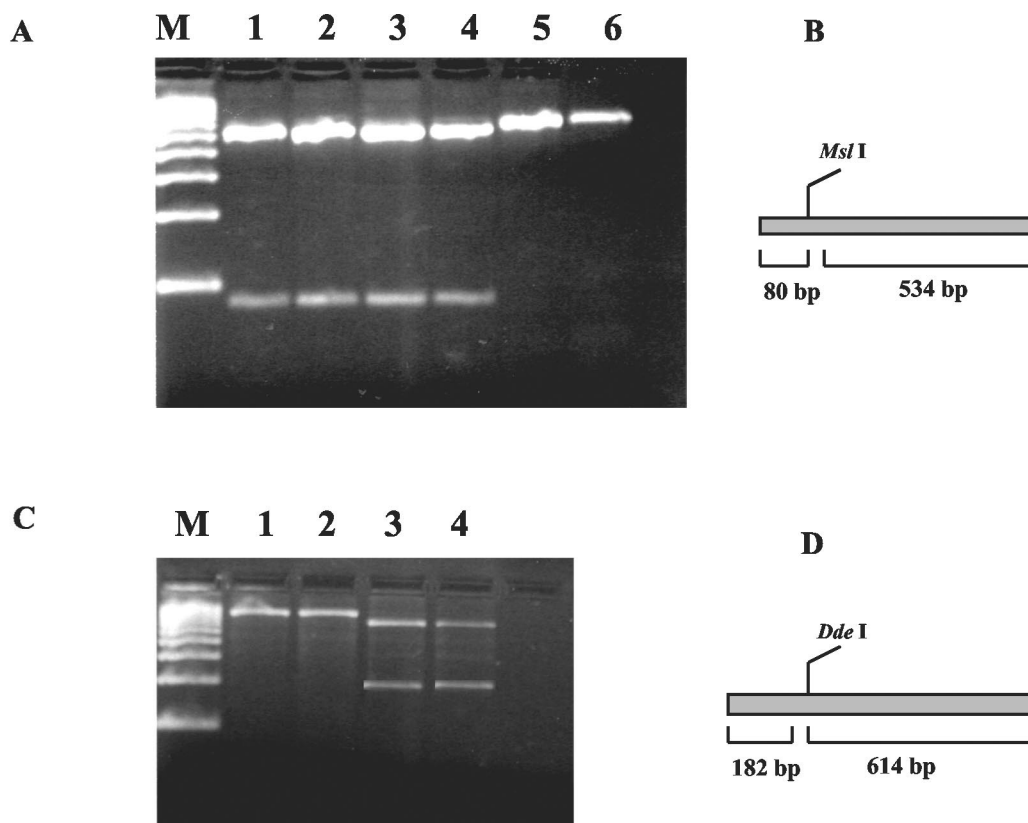
FIG. 3. Enzyme restriction mapping. (A and B) A 614-bp PCR product from the 16S rRNA gene cleaved with restriction enzyme Mst I. (A) Gel separation. (B) Restriction map. (C and D) A 796-bp product from the hsp65 gene cleaved with restriction enzyme Dde I. (C) Gel separation. (D) Restriction map. Lanes: M, 100-bp molecular size marker; 1, DL240490; 2, SR030597; 3, CC240299; 4, BB170200; 5, ATCC 927; 6, DLDK.
