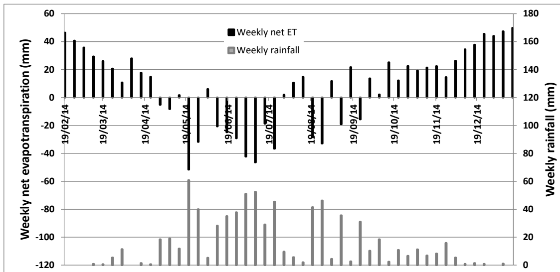
Figure 2. Weekly net evapotranspiration and rainfall totals (mm) for the summer and winter drying trial periods.
