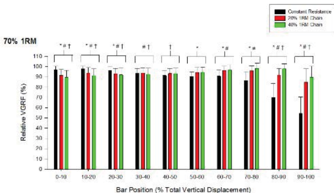
Figure 4: Force produced during deadlifts performed with a constant resistance and chains
