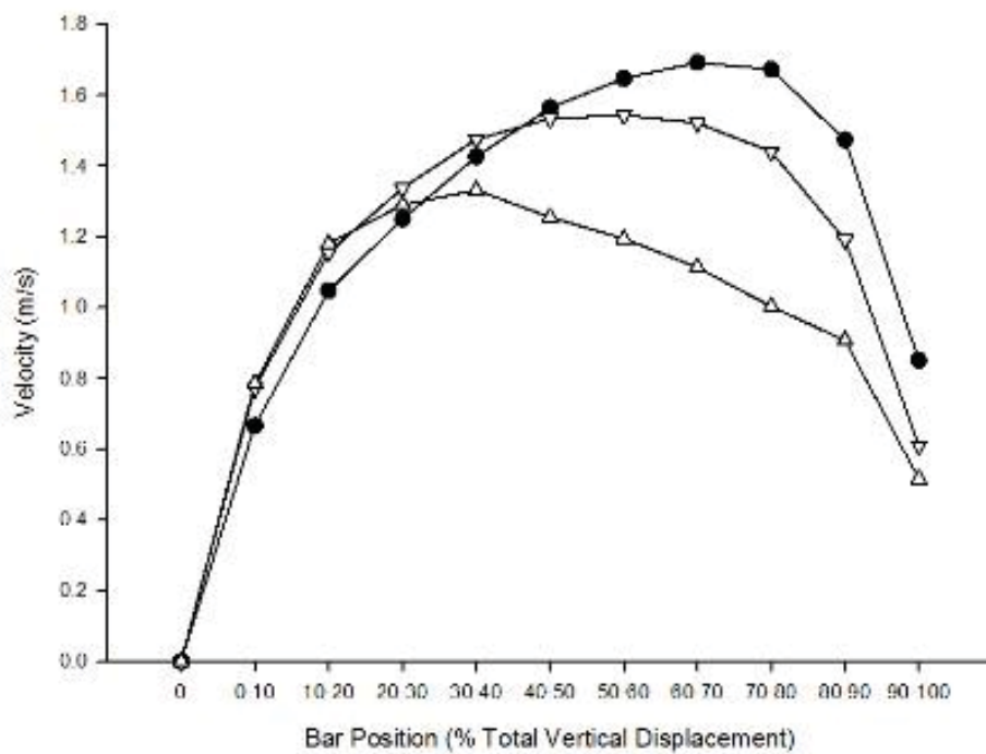
Figure 10: Velocity produced during deadlifts performed with a constant resistance and chains.
