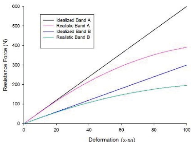
Figure 7: Comparison of idealised and realistic force-deformation curves for resistance bands
